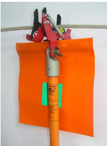
FLAG part no. 1059 open snap clamp being fitted with hot stick and red tool.
